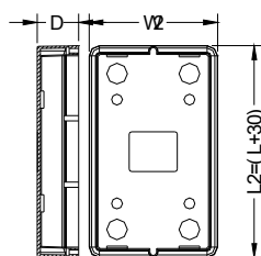
Side and back view of back cover
