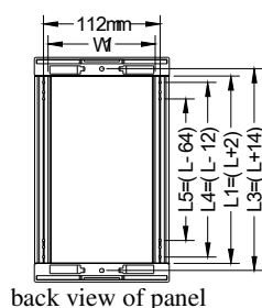
back view of panel
